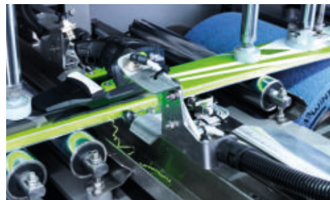
Trimcut automated sidewall pretreatment
