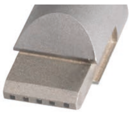
Diamond dresser Rhomboid 5 x 0,5 x 0,5 mm RC, Total bearing surface 1,25 mm², r = 0,33 mm
