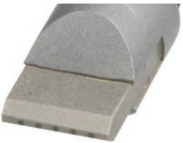
Diamond dresser Rhomboid 5 x 0,5 x 0,5 mm RC, Total bearing surface 1,25 mm², r = 0,33 mm
